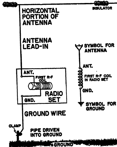
Receiving antenna, with schematic symbol and names of important parts.
